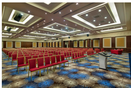
Gaia
